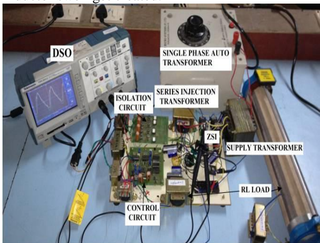
Fig. 8. Overview of the Hardware Setup
