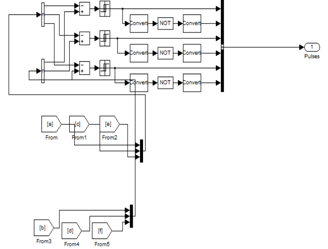
Fig. 5 Hysteresis Controller
