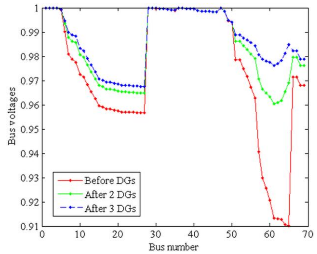
Figure 7. Improved voltage profile of 69 bus system
