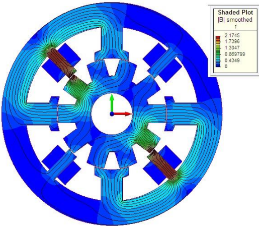
Fig.2. Phase B Excitation and its Flux Path
