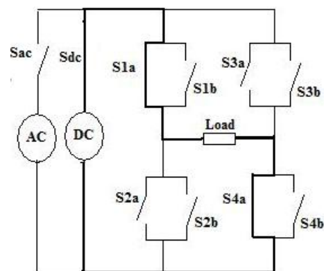
FIG.5: Switching states as Chopper
