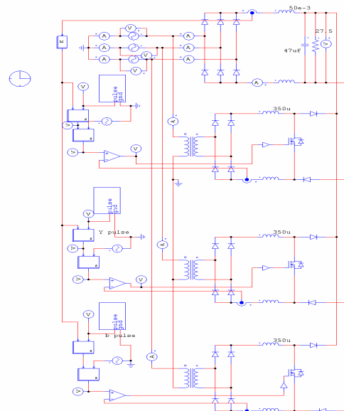
Fig. 21 Psim schematic diagram of sinusoidal source current
