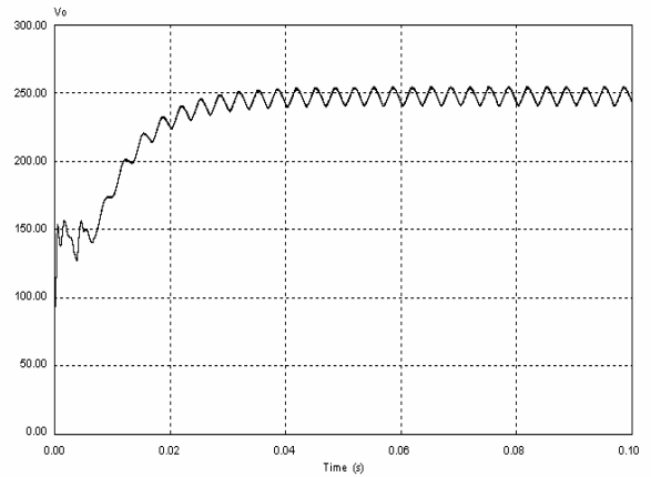
Fig. 10 Output voltage of 12 Pulse HMPR
