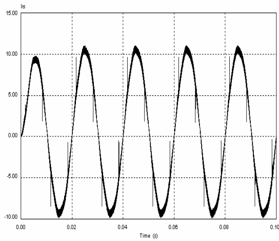
Fig.17 R_{ph} Source Current ( I_{rs} )
