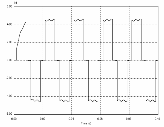
Fig. 15 Diode Bridge R_{nh} Line current I_{rh}
