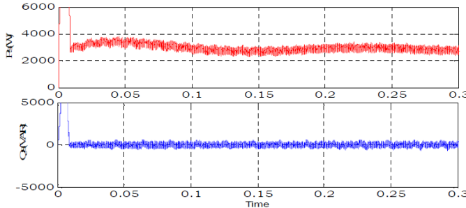
Figure 6 (b): waveform of instantaneous powers after SAPF commissioning.
