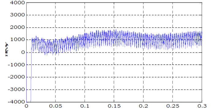
Figure 10: waveform of the active power injected into the grid by the PV Generator.
