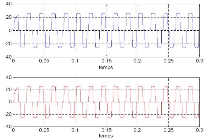
Figure 4 (a) current waveforms before photovoltaic compensation.
