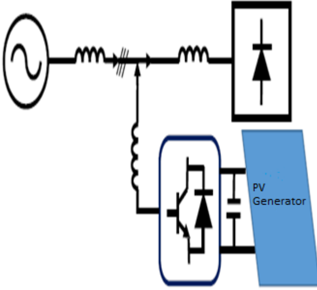
Figure 1: Synoptic diagram of the configuration studied
