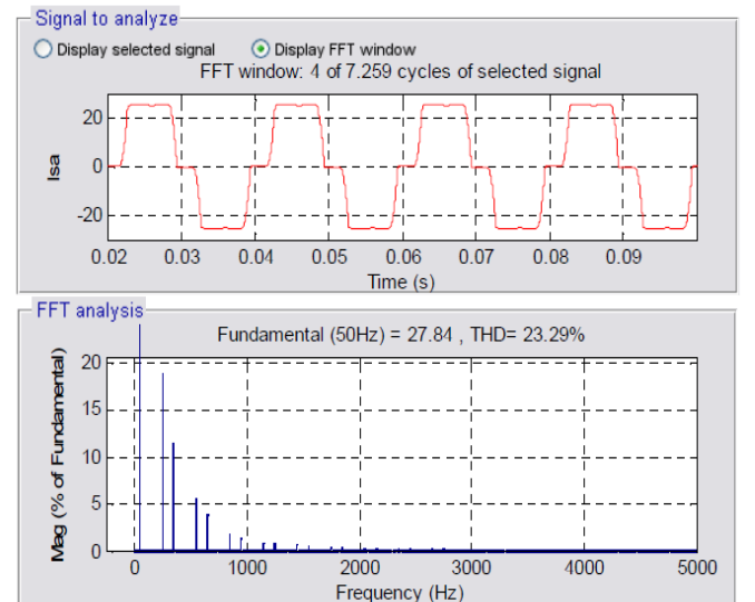
Figure 5: Spectral analysis of the source current before commissioning of the SAPF.
