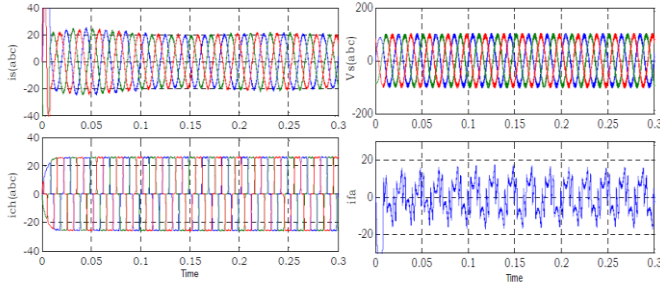
Figure 6 (a): Transient simulation results when closing the SAPF for a PD3- [RL1, L] nonlinear load.
