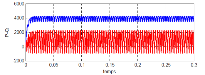
Figure 4(b): Active and reactive power characteristic.
