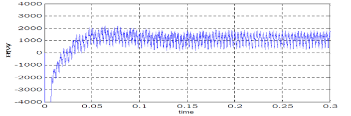
Figure 14: waveform of the active power injected into the grid by the PV Generator (DPC).
