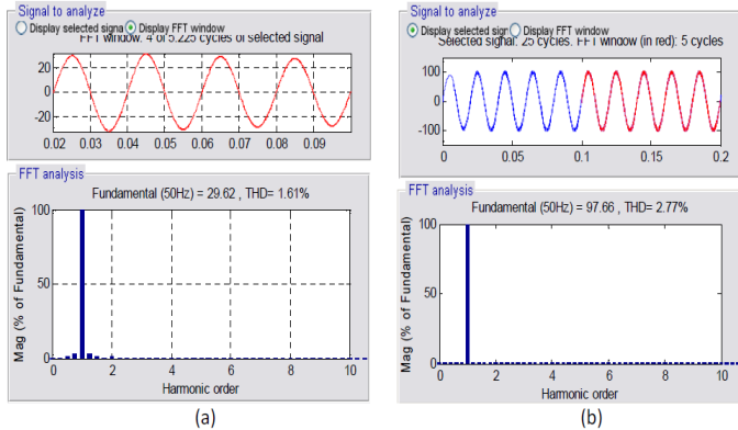
Figure 12: Spectral analysis of the signals after SAPF commissioning: (a) source current, (b) source voltage (DPC).
