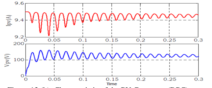
Figure 13 (b): Characteristic of the PV Generator (DPC).
