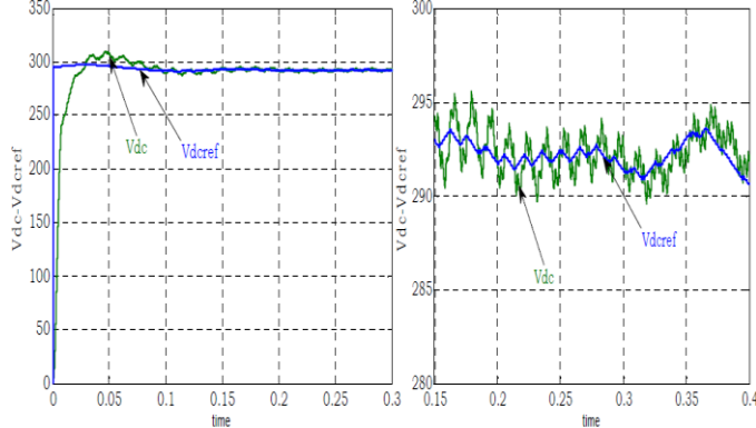
Figure 13 (a): waveform of the DC bus voltage and its reference voltage (DPC).
