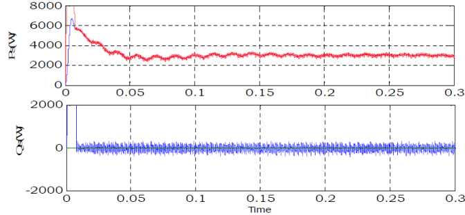
Figure 11 (b): waveform of instantaneous powers after SAPF commissioning (DPC).
