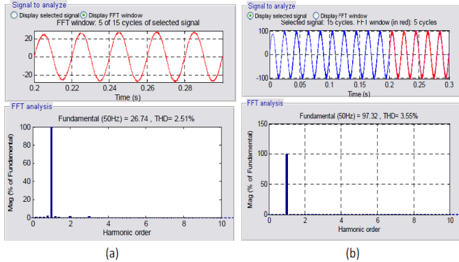
Figure 7: Spectral analysis of signals after SAPF commissioning: (a) source current, (b) source voltage.
