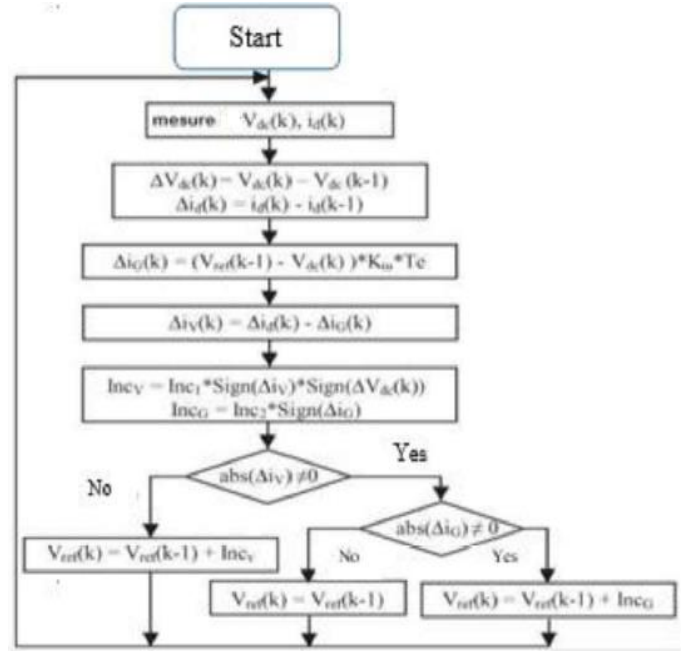
Figure 3: Proposed MPPT algorithm for estimating the reference voltage.
