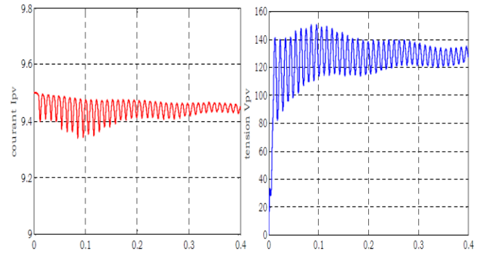
Figure 9: Characteristic of the PV Generator.
