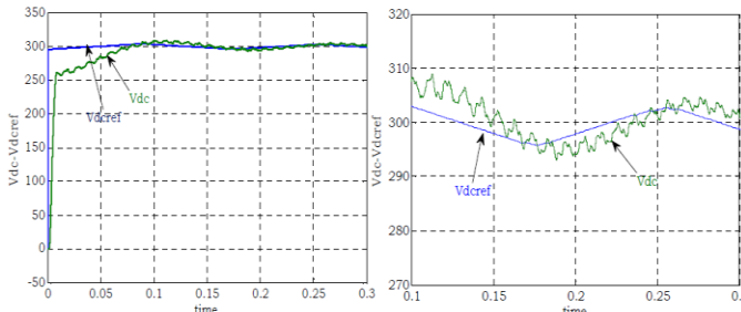
Figure 8: waveform of the DC bus voltage and its reference voltage.
