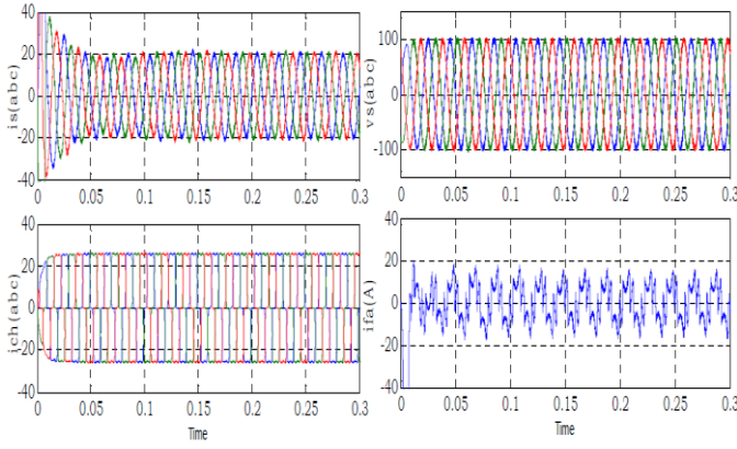
Figure 11 (a): Transient simulation results at closure of SAPF for a PD3- [RL1-L] nonlinear load.
