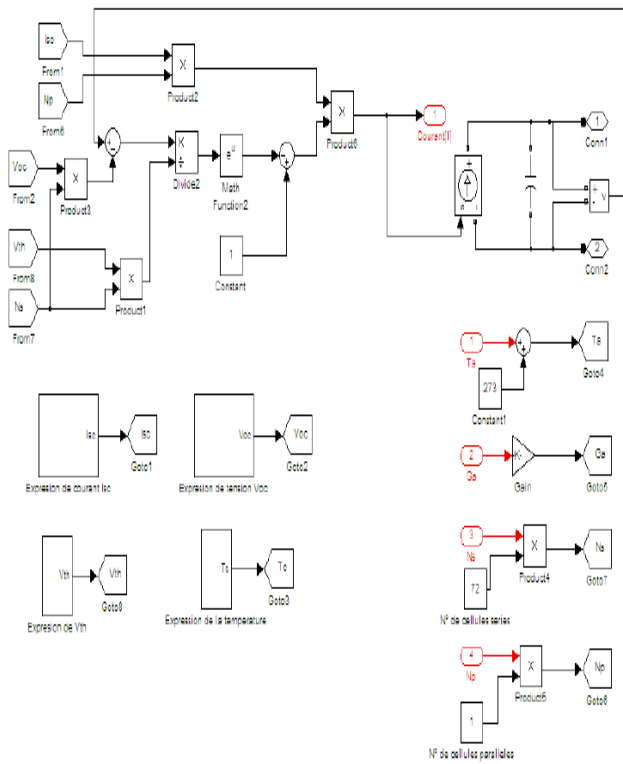
Figure 2: Modeling PV generator under matlab-Simulink.
