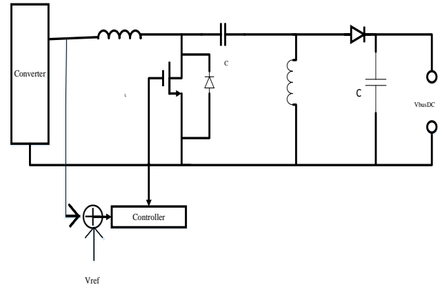
Figure: 3 Photovoltaic conversions with input voltage controller
