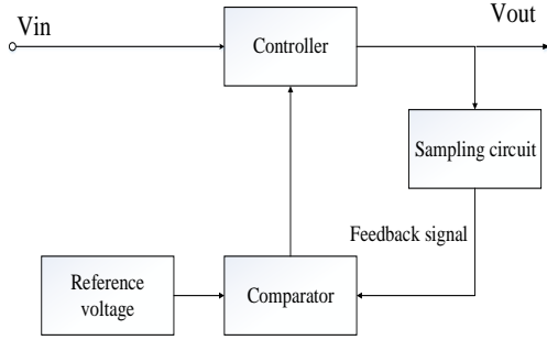
Figure 4: Voltage regulator
