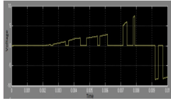
Figure 11: Regulator voltage
