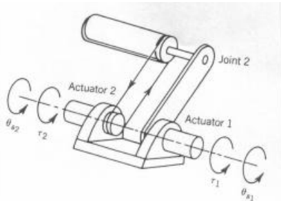
Fig. 1: Two link revolute joint arm with remotely driven link
