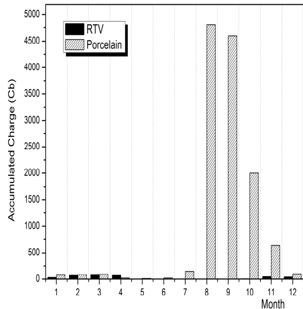
Fig.4. Monthly distribution of the accumulated charge, given as the maximum value in the nine years monitoring period, for the RTV SIR coated porcelain coated insulators.
