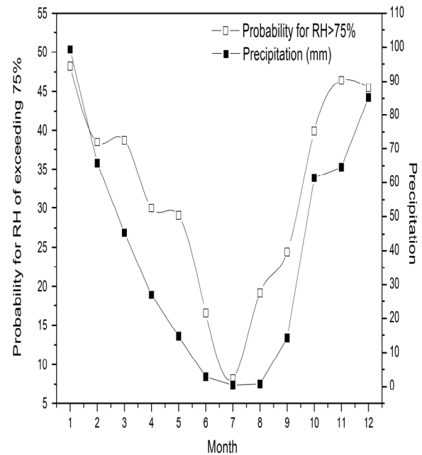
Fig.6. Average precipitation and probability for relative humidity to exceed 75% per month (data available after a 20 years monitoring period).
