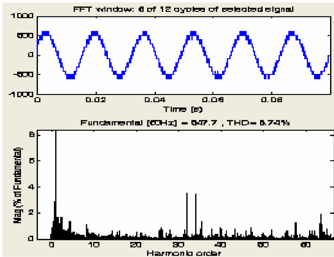
Fig.10. Output Line Voltage of Seven Level Inverter and its FFT analysis for m_i = 0.8
