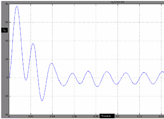
Fig.9. Output line current to IM load for m_i = 0.8 of seven-level inverter
