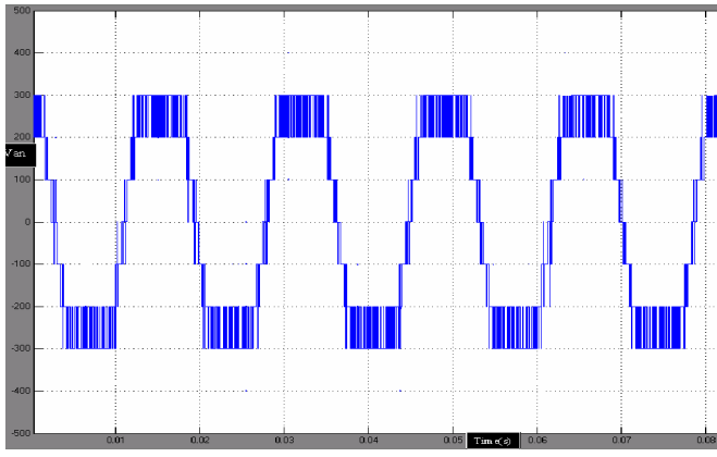
Fig.8. Output Phase Voltage of Seven-level inverter for modulation index ( m_i ) = 0.8
