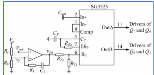
Fig 14.driver circuit
