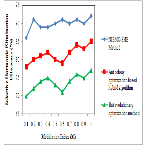
Figure 11 Measure of SHE Efficiency
