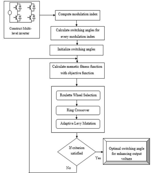
Figure 1 Architecture diagram of NIEMO-SHE Method
