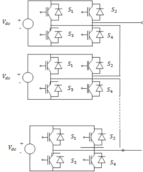
Figure 2 Circuit Diagram of Multilevel Inverter
