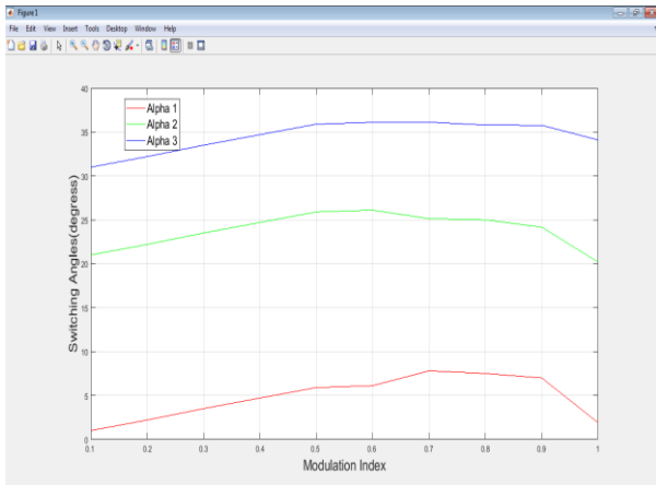
Figure 8 Switching angles (degrees) for different Modulation Index
