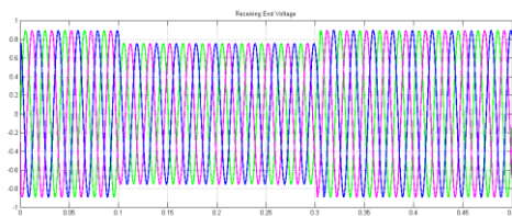
Fig 22. Voltages sag by inclusion of inductive load at 0.1 sec and removal of inductive load at 0.3 sec without STATCOM
