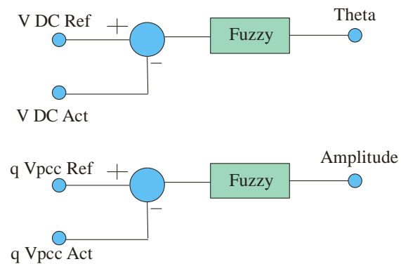
Fig 6. FLC controller
