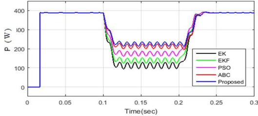
Figure. 20 Real Power Comparison at BC fault
