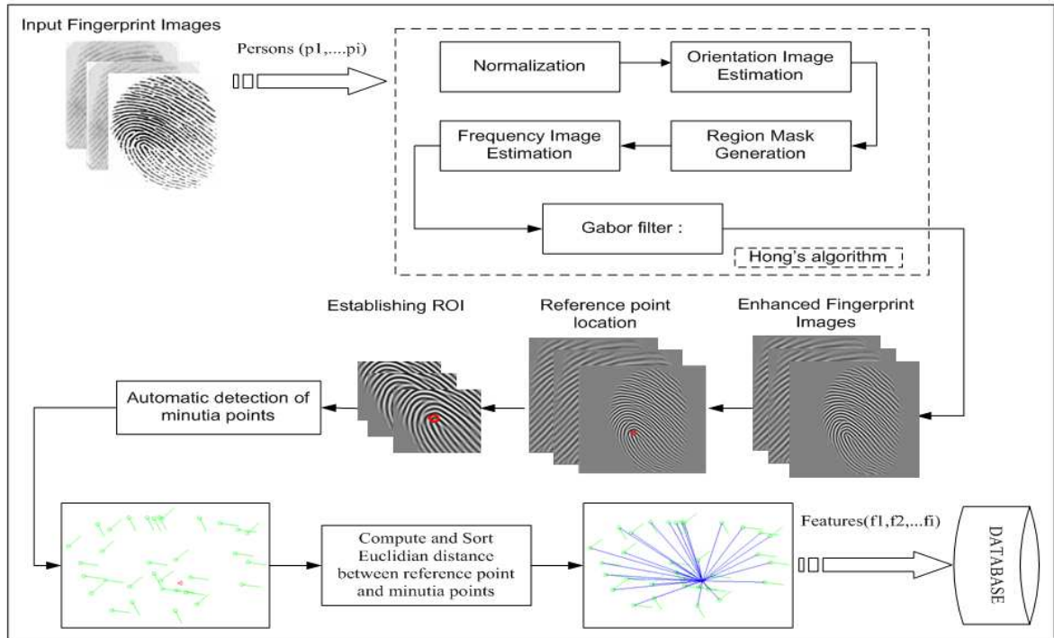
Fig. 6. Flowchart of fingerprint enhancement algorithm, locating reference point and proposed fingerprint matching approach
