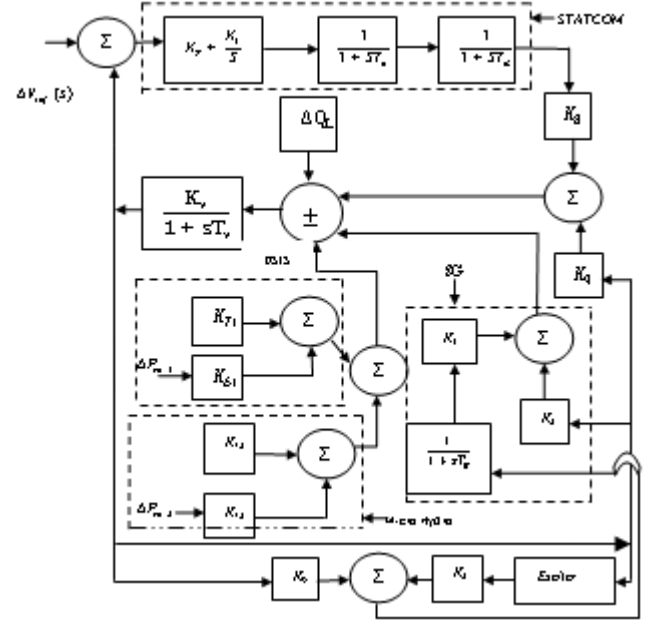
Figure 2. Block Diagram of Isolated Hybrid Energy System
