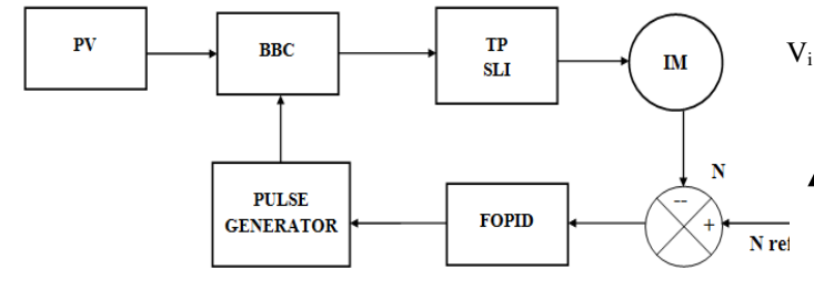
Figure 2: Block Diagram of Proposed BBCTPSLI System
