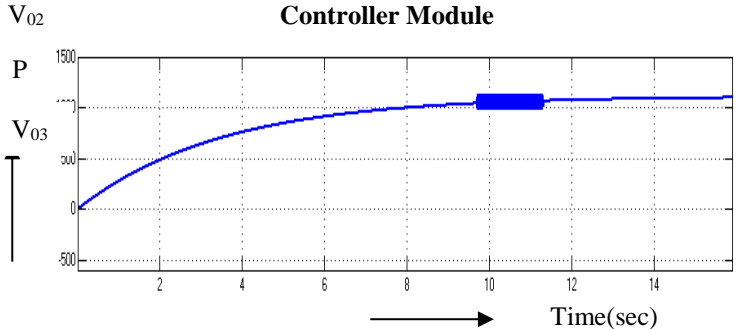
Figure 3.4: Motor Speed of BBCTPSLI System with PI Controller Module
