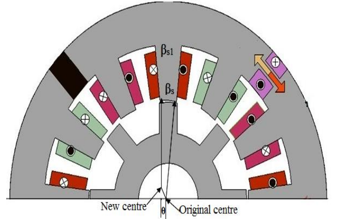
Fig.11. HSRM with stator pole tapering and non uniform air gap
