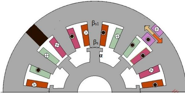
Fig. 14. HSRM with stator tapering and pole shoe at rotor
