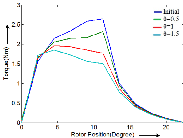
Fig. 6. Torque characteristics of HSRM with non uniform air gap
