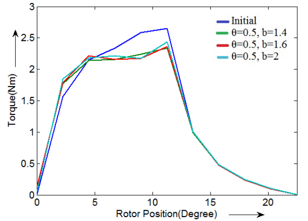
Fig.12. Torque characteristics of HSRM with stator pole tapering and non uniform air gap
