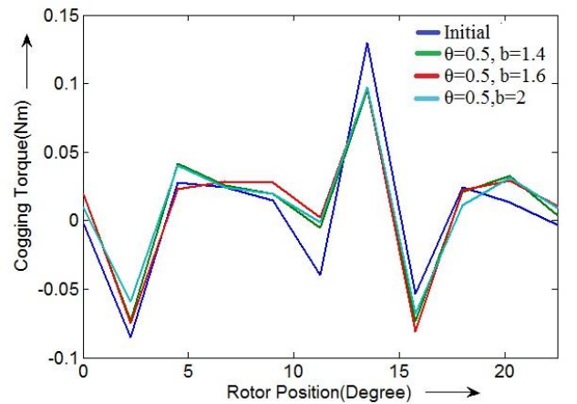
Fig. 13. Cogging torque characteristics of HSRM with stator pole tapering and non uniform air gap
