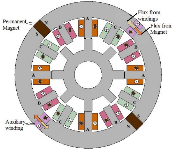
Fig. 1. Structure of HSRM
