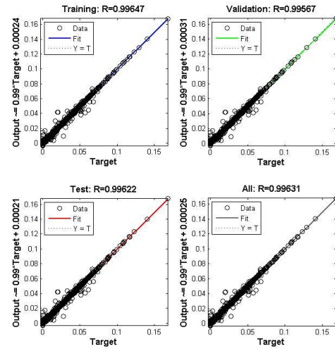
Fig.5.7 regression graphs
