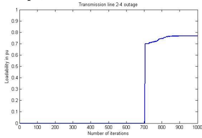
Fig.5.4 transmission line 2 – 4 outage Table 5.2 Individual Load Bus maximum loading
