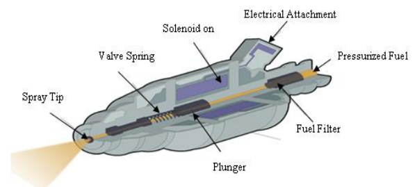
Fig.1. Design of Fuel Injector
