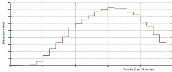
Fig. 10. The sampled radiation data on July, 1, 2016
