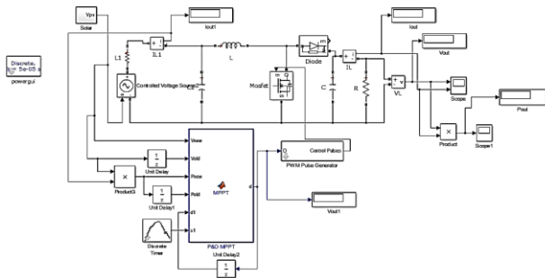
Fig. 8. Simulink block diagram of improved dp P&O method
