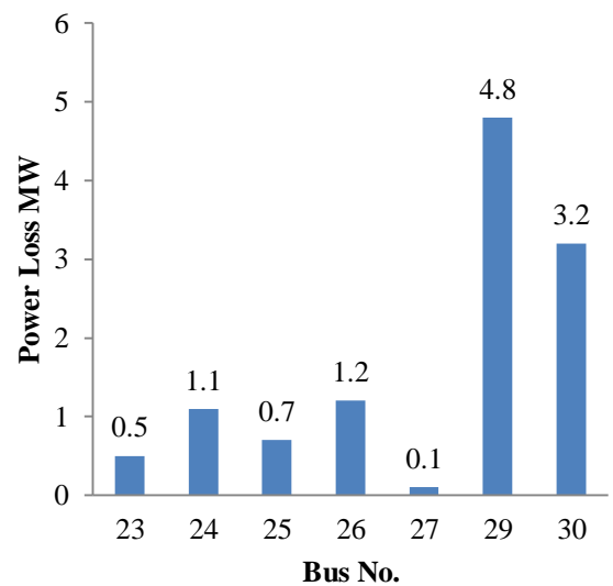
Fig.10 MW loss load area 4
