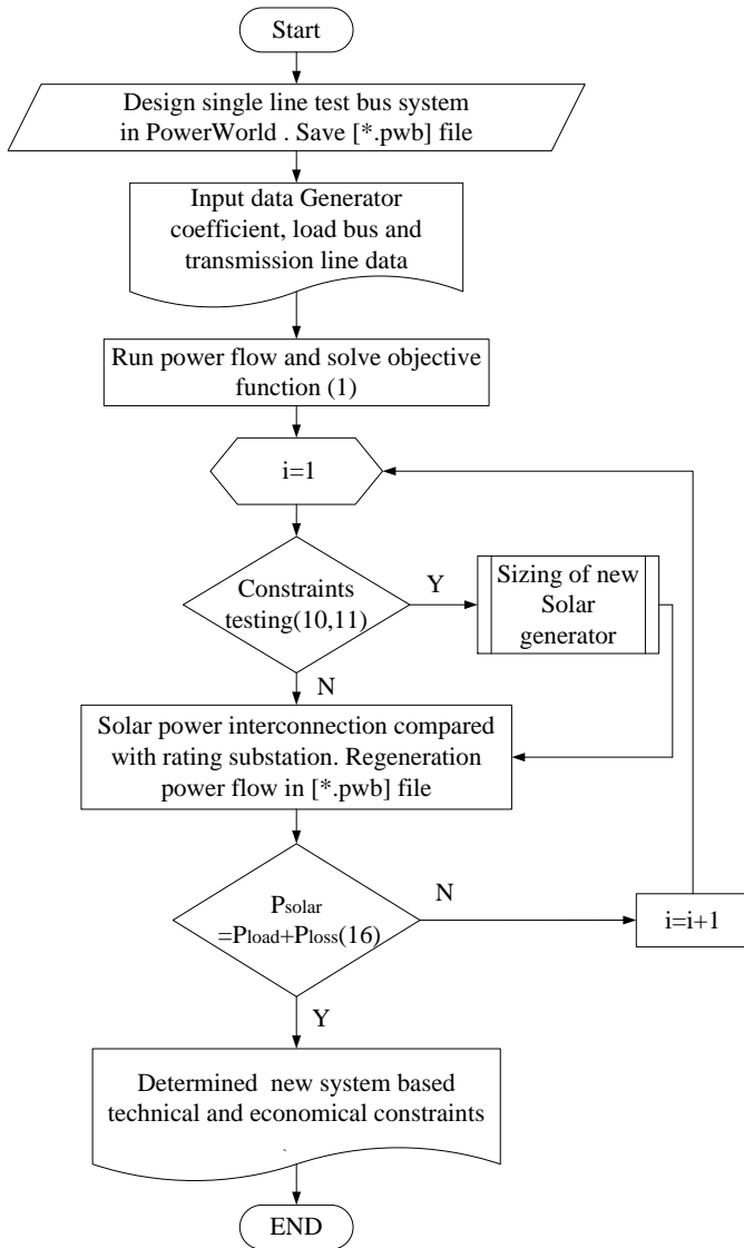
Fig.6. Proposed algorithm flow chart
