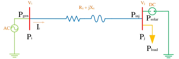
Fig.5. single line diagram of between two buses.
