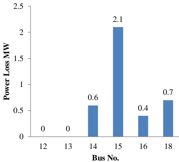
Fig.8 MW loss load area 2
