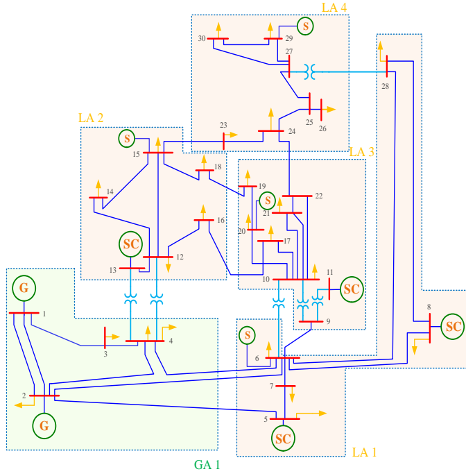
Fig.1. Planned to interconnection of solar energy generator IEEE 30-bus system.
