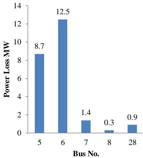
Fig.7 MW loss load area 1
