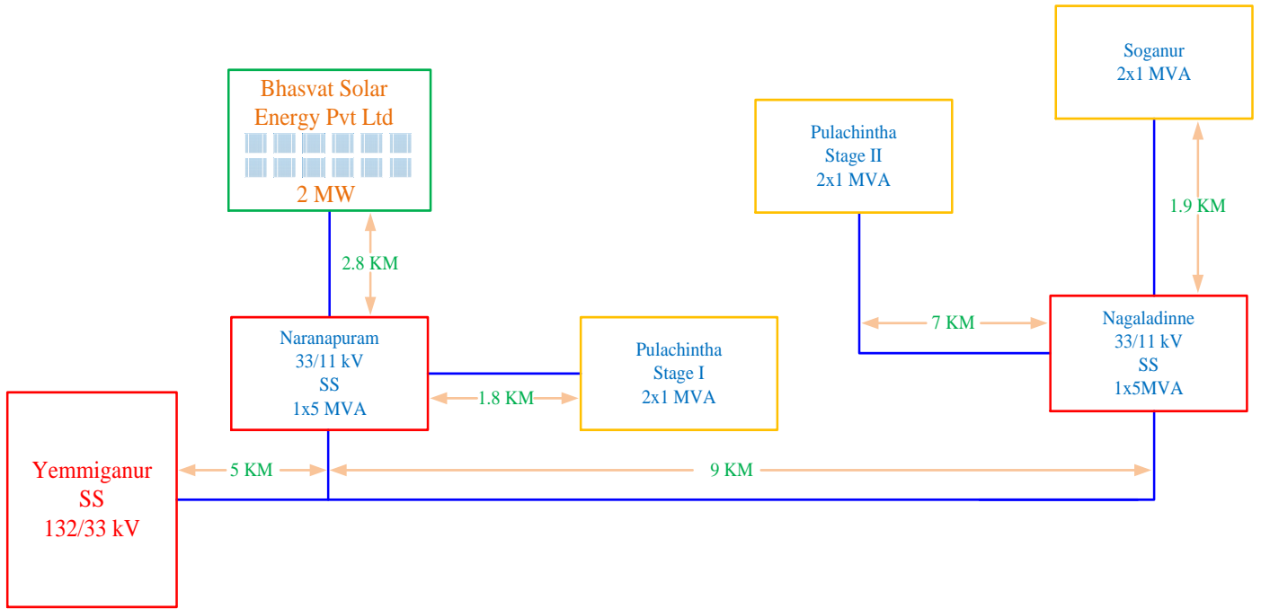
Fig.11. single line diagram EHT SS 33/11 kV with solar power plant.
