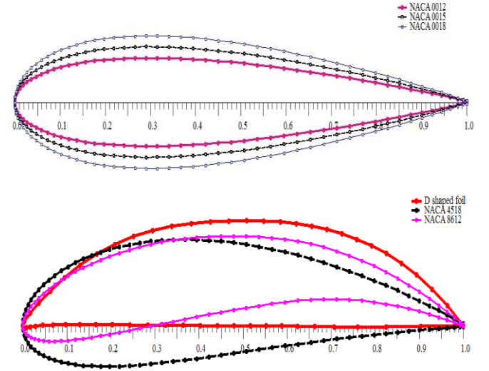
Fig 4. NACA symmetrical and unsymmetrical Airfoil shapes and a D shaped foil
