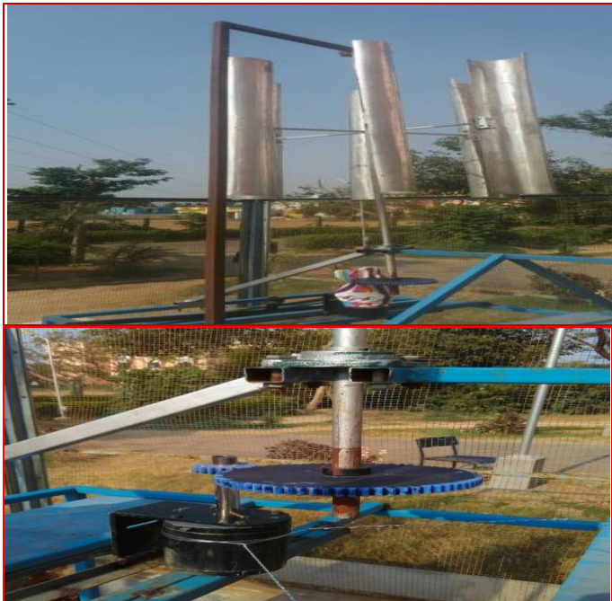
Fig 21.VAWT model with Aspect Ratio= 2.5 with PMDC Generator 1:7 gear ratio Assembly.
