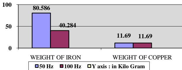
Fig. 7.5. Comparison of 50Hz and 100Hz DVR Injection transformer for the Weight of iron and Weight of copper
