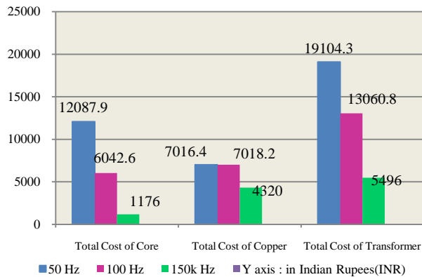
Fig. 7.8. Cost Comparison of 50Hz, 100 Hz and 150k Hz DVR Injection transformer for the Total Cost of Core, Total Cost of Copper and Total Cost of DVR Injection transformer
