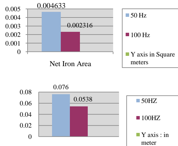
Fig. 7.1. Comparison of 50 Hz and 100 Hz DVR Injection transformer for the (a) net iron area (b) diameter of the circumscribing circle
