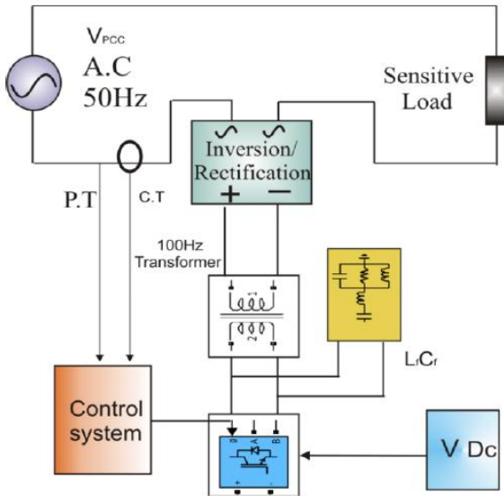
Fig. 2. Proposed DVR arrangement
