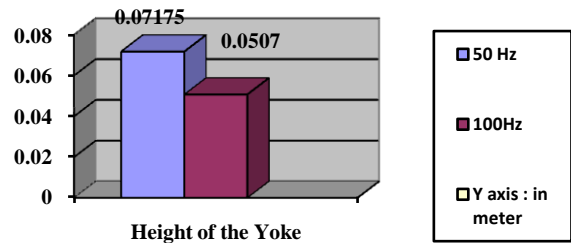
Fig. 7.3. Comparison of 50Hz and 100Hz DVR Injection transformer for the (a) Depth of the yoke (b) Height of the yoke
