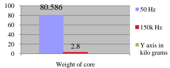
Fig. 7.7. Comparison of 50Hz and 150k Hz DVR Injection transformer for the Weight of the core
