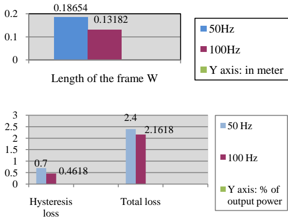
Fig. 7.4. Comparison of 50Hz and 100Hz DVR Injection transformer for the (a) Length of the frame 'W' (b) Hysteresis and Total losses
