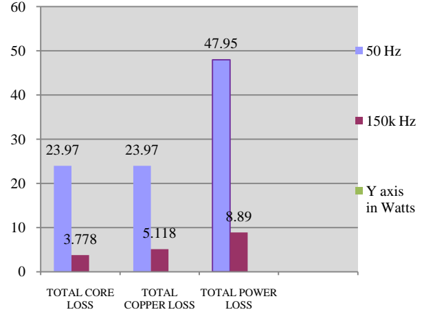
Fig. 7.6. Comparison of 50Hz and 150k Hz DVR Injection transformer for the Total core loss, Total copper loss and Total power loss
