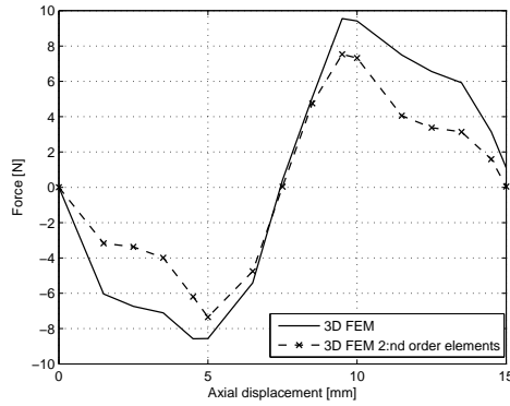
Fig. 10. 3D-simulated force for one phase magnets.
