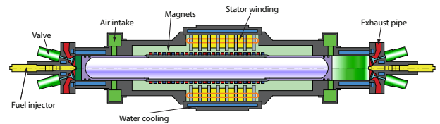
Fig. 1. Schematic view of the FPEC.
