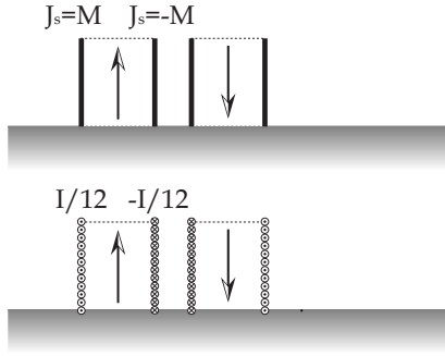
Fig. 6. Simplified TFM configuration in the w coordinate system.
