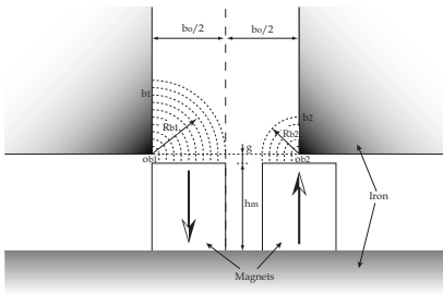
Fig. 3. Idealized flux path used for calculation of the permeance.
