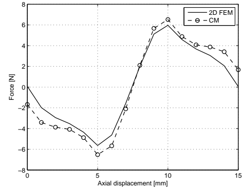
Fig. 8. Force for one tooth.
