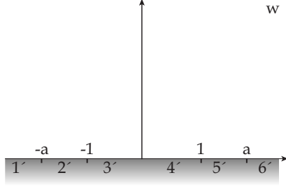
Fig. 6. Simplified TFM configuration in the w coordinate system.
