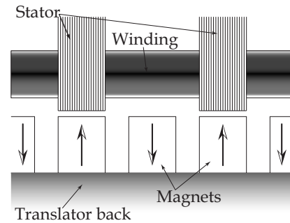
Fig. 2. Layout of the new TFM design
