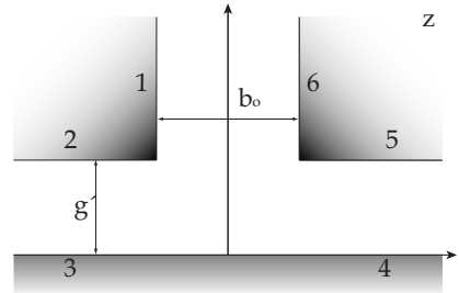
Fig. 5. Simplified TFM configuration in the z -plane.
