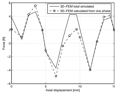
Fig. 11. 3D-simulated force for all phases and calculated results from 3D-FEM results for one phase.
