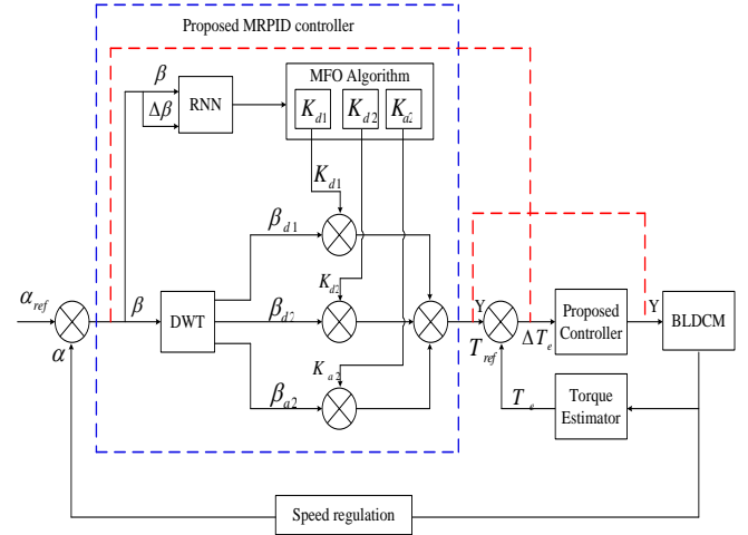
Figure.2: Proposed RNN- MFO based MRPID controller
