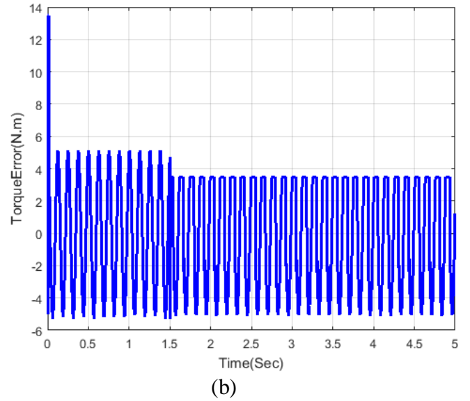
Figure 10: Evaluation of (a) speed and (b) torque error values in case 3
