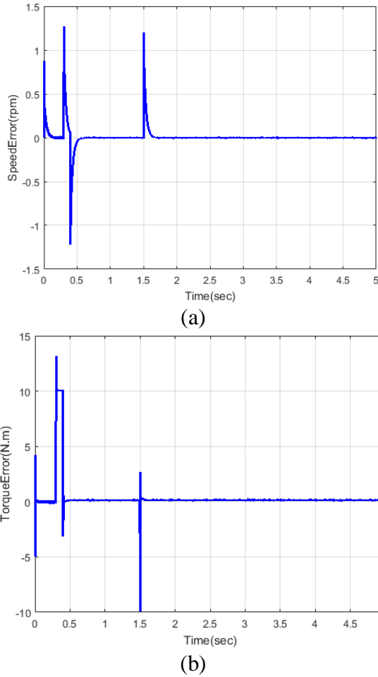
Figure 8: Performance analysis error values in case-2 (a) speed and (b) torque
