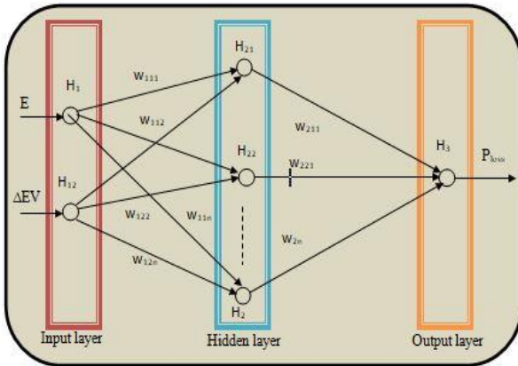
Fig.3: Proposed RBFNN layers representation
