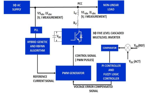
Fig.1: Proposed CHBMLI based Shunt APF block diagram
