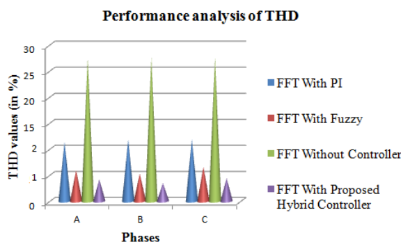
Fig.10: THD analysis with different control technique
