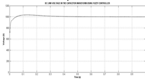
Fig.6(b): Capacitor DC link voltage using fuzzy compensation
