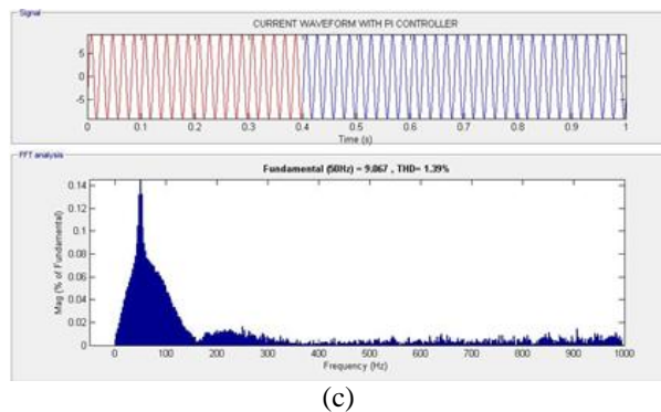
Fig.9: THD values for proposed controller, PI and Fuzzy logic controller
