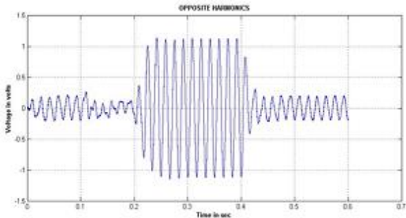
Fig.7: Voltage injected in the PCC with three phase five level inverter
