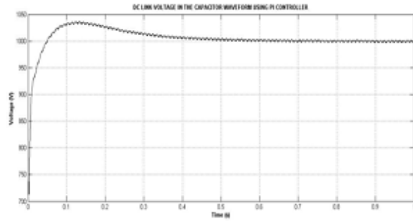
Fig.6(a): Capacitor DC link voltage using PI compensation
