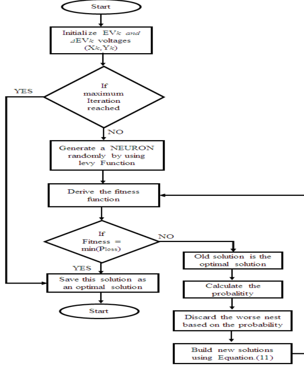
Fig.2: Flow chart for proposed hybrid algorithm
