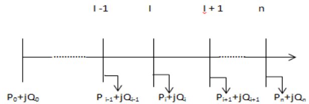
Fig. 1. Single line diagram of a distribution network
