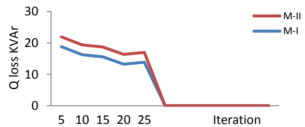
Fig. 10. Comparison of reactive power loss curves the 62 bus
