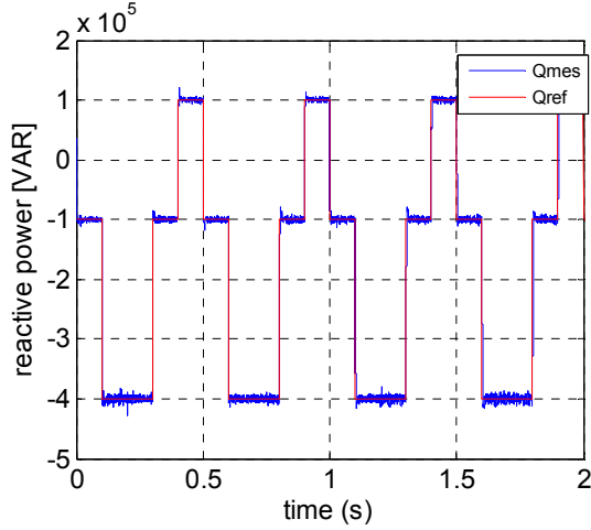
Fig.14. Electrical reactive power produced with SVM.
