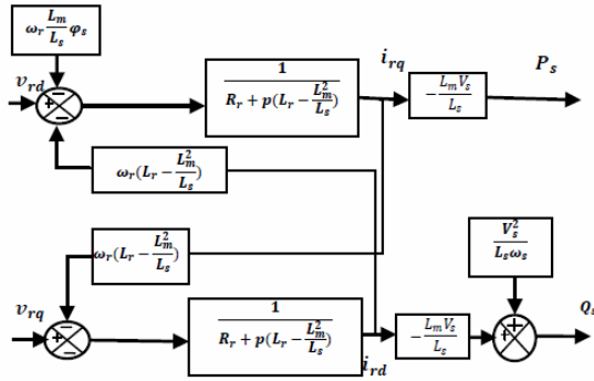
Fig.3. Block diagram of the DFIG model.
