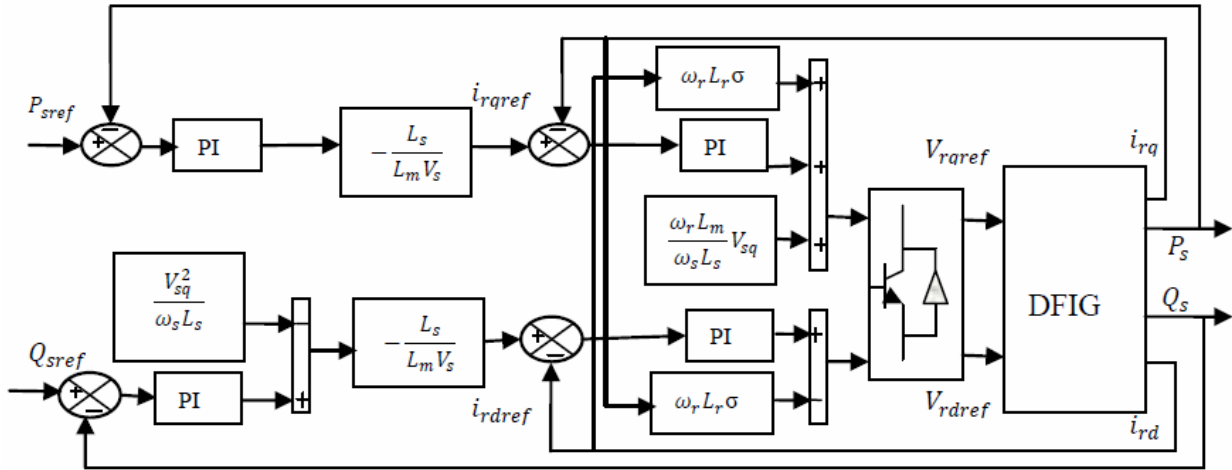
Fig.4. Schema block indirect regulation with loop power
