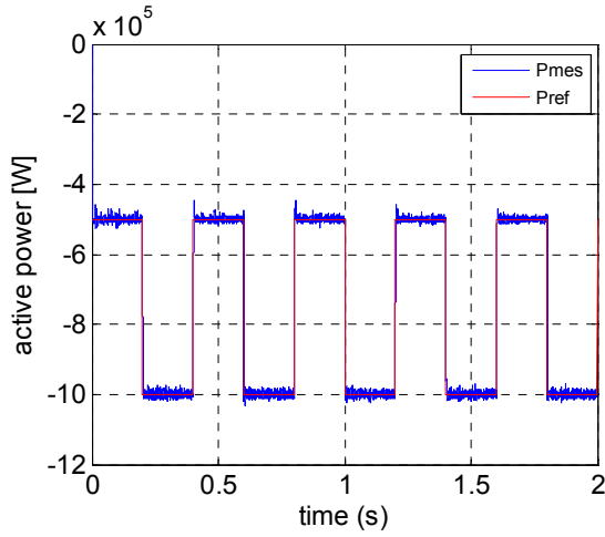
Fig.13. Electrical active power produced with SVM
