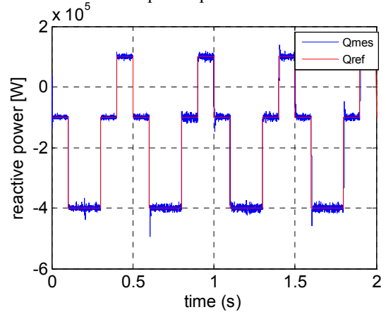
Fig.8. Electrical reactive power produced with PWM.
