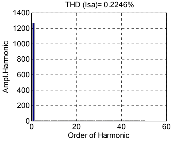
Fig.10. THD of current I_{s\alpha} with PWM .
