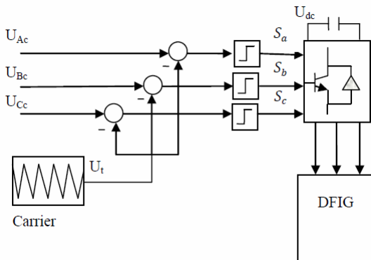
Fig.6. Block scheme of carrier based sinusoidal PWM
