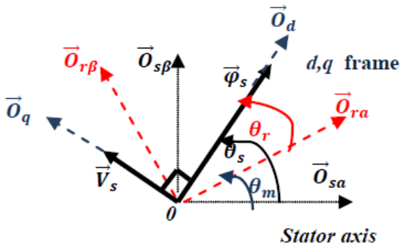
Fig.2. Determination of the electrical angles in Park reference frame.
