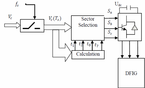
Fig.12. Block scheme of the space vector modulator
