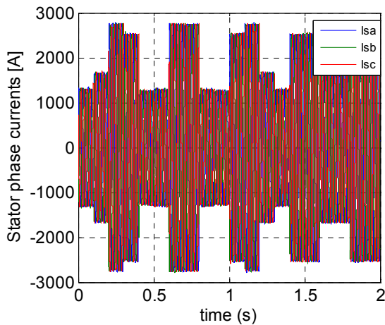
Fig.15. Stator phase currents with SVM
