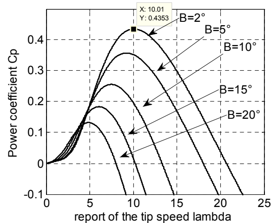
Fig. 1. The power factor for different angles of stalls.
