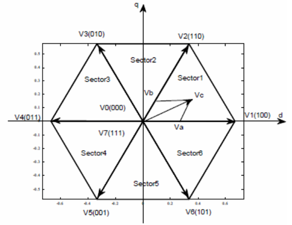
Fig.11. Principle of the space vector modulation
