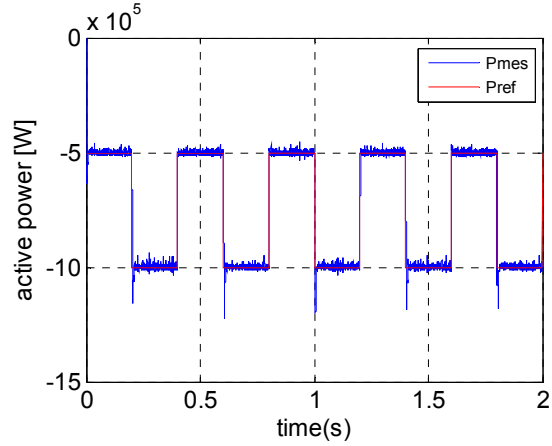
Fig.7. Electrical active power produced with PWM.
