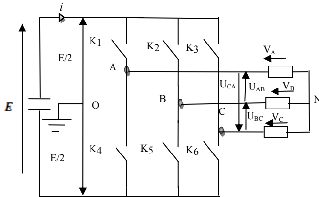
Fig.5. Simplified diagram of the three-phase inverter.
