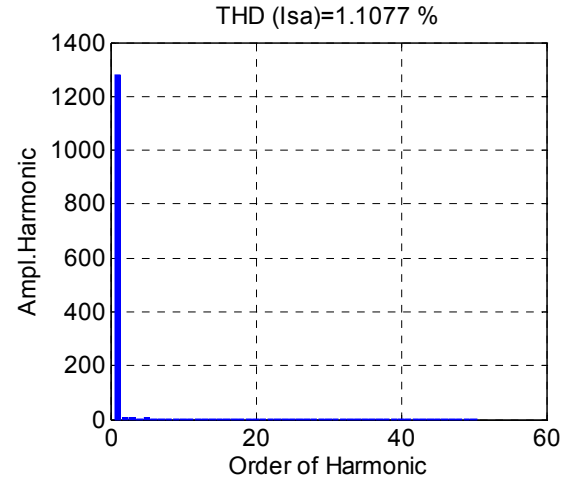
Fig.16. THD of current Isa with SVM.
