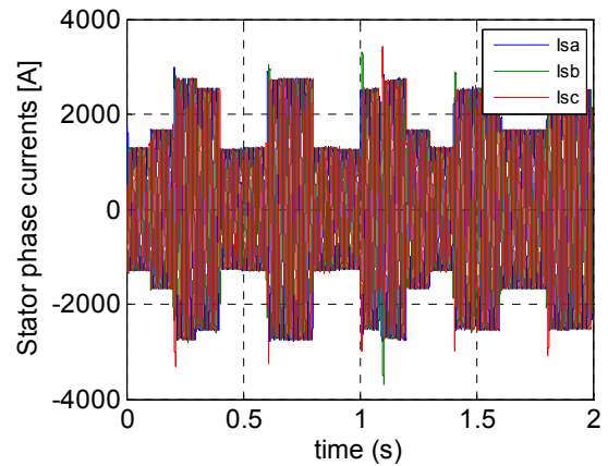
Fig.9. Stator phase currents with PWM
