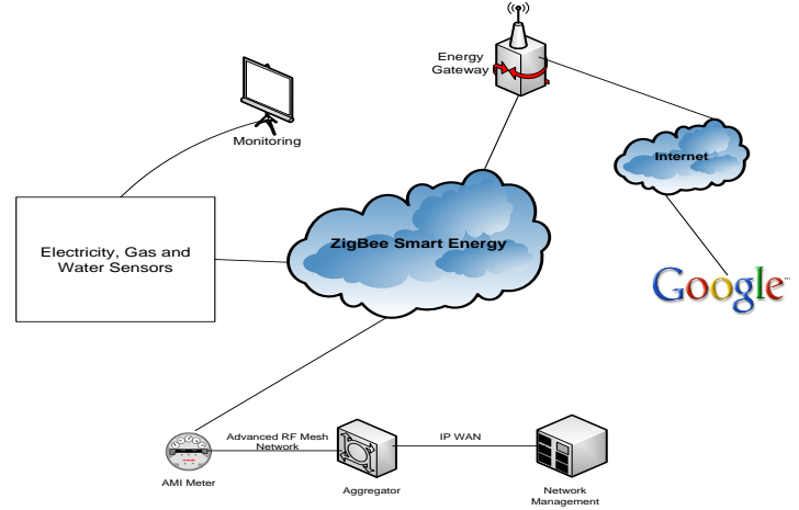
Figure 4 Data Communication of AMI using ZigBee
