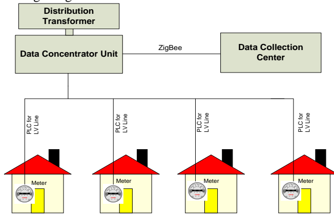
Figure 6 Hybrid Systems for AMI
