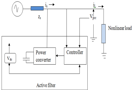
Figure.2 Block Diagram of Shunt Active Power Filter
