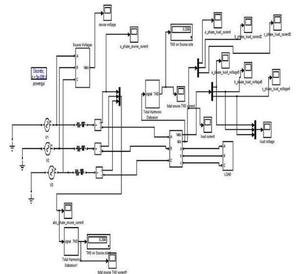
Figure.8 Three Phase Power System without Filter in MATLAB
