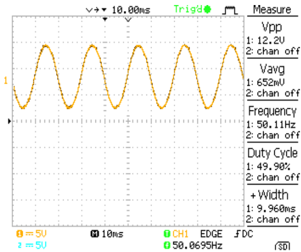
Fig.16. Voltage across capacitors V_{C1} .
