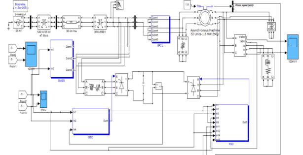
Fig.12. DFIG with SFCL and SMES for Voltage regulation and Fault current limitation
