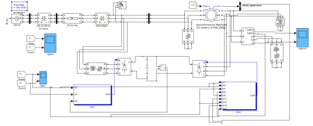
Fig.8. Modelling of DFIG based wind power generation under fault
