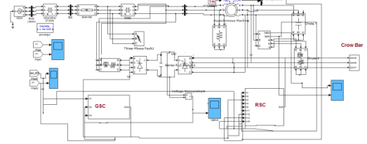
Fig.10. Conventional method for protection (Crow bar protection Scheme).
