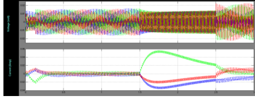
Fig.13.Voltage and Current in Stator and Grid Under faulted condition.
