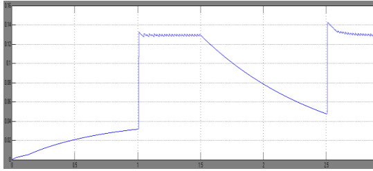
Fig.15.Capacitor Voltage
