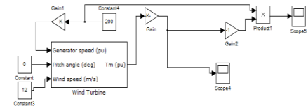
Fig.9. Torque Generation
