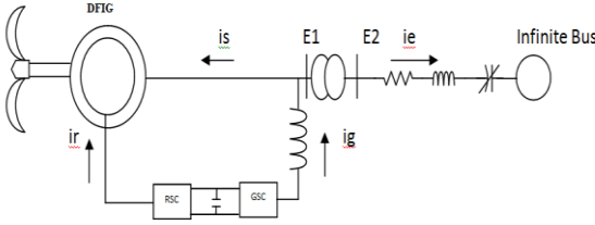
Fig. 1. Wind turbine model
