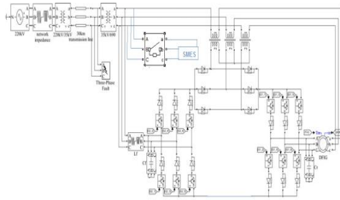
Fig.7. DFIG incorporated with the SFCL-MES (voltage source topology)
