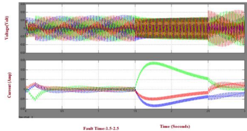
Fig.17.Limited Rotor voltage and current by the effect of SFCL
