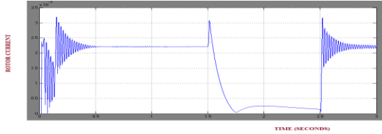
Fig.16 Rotor Fault current under conventional control technique.
