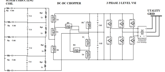
Fig. 5. Detailed model of the proposed SMES system including the PCS and the SC.
