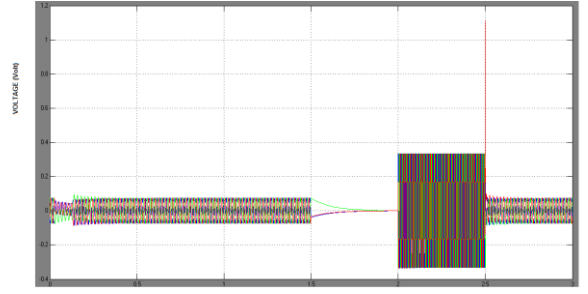
Fig.18. Stator Voltage by the action of SMES
