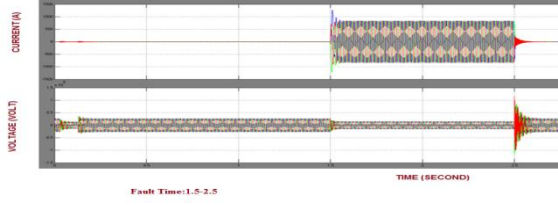
Fig.13.Voltage and Current in Stator and Grid Under faulted condition.
