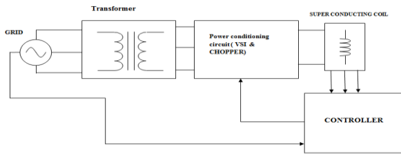
Fig. 4. Components of a typical SMES system
