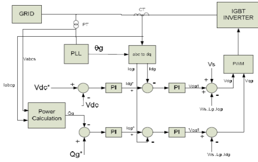
Fig. 3 The Grid-Side Converter (GSC)
