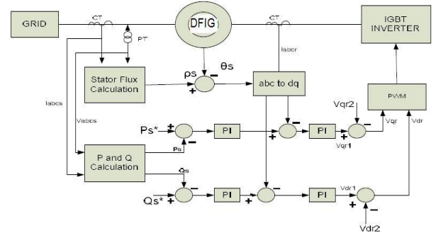
Fig. 2 The Rotor-Side Converter (RSC)
