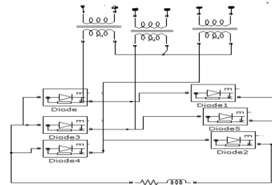
Fig.11. Bridge Type SFCL
