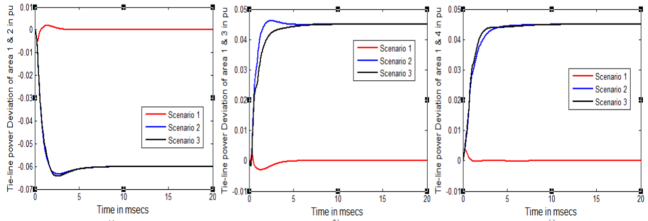
Fig. 7 Tie line power deviation between (a) area 1 & 2 (b) area 1 & 3 (c) area 1 & 4
