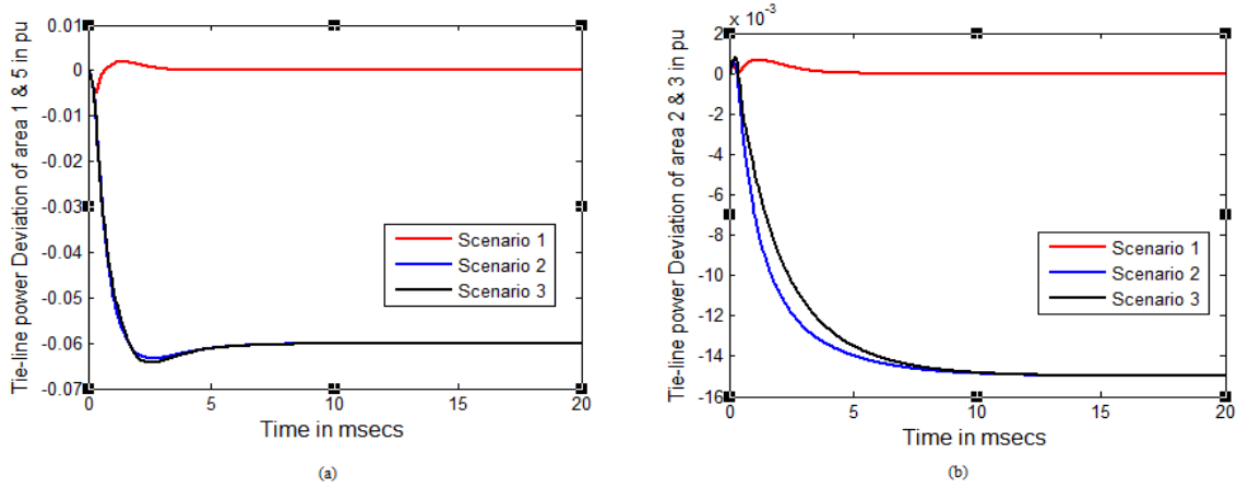
Fig. 8 Tie line power deviation between (a) area 1 & 5 (b) area 2 & 3
