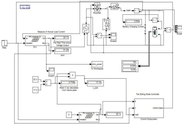
Fig. 6a Simulation Diagram of Sliding mode Controller
