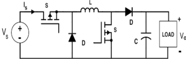
Fig. 4 Schematic Diagram of Non Inverting Buck-Boost Converter
