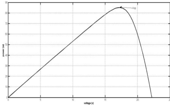
Fig. 3 b) P-V Characteristics of a PV module for 1000W/m 2
