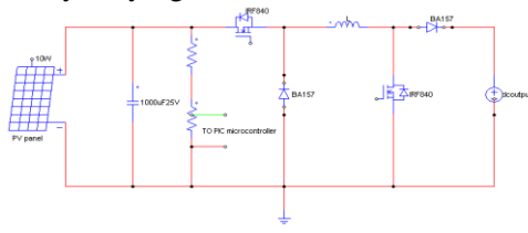
Fig 11. Circuit Diagram of Proposed System
