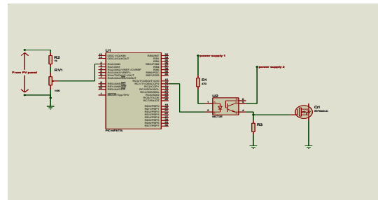
Fig 12. Circuit Diagram of Control Circuit with PIC 16F877A
