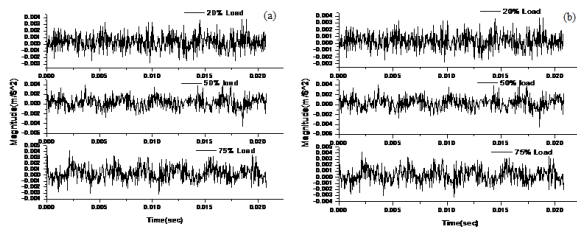
Fig.12 Measured vibrations under different load conditions at 1000 rpm
