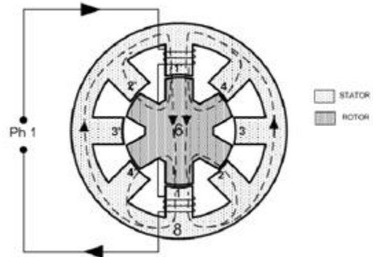
Fig.1. Cross-sectional view of 4 Phase SRM
