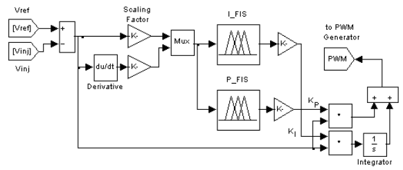
Fig. 7. SIMULINK model of the proposed controller
