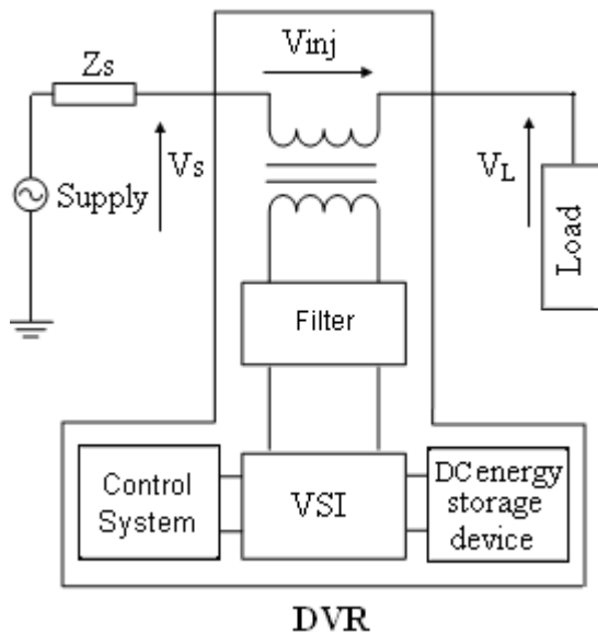
Fig. 1. DVR general configuration
