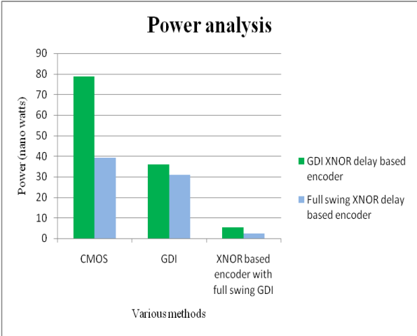
Fig.15 Power analysis
