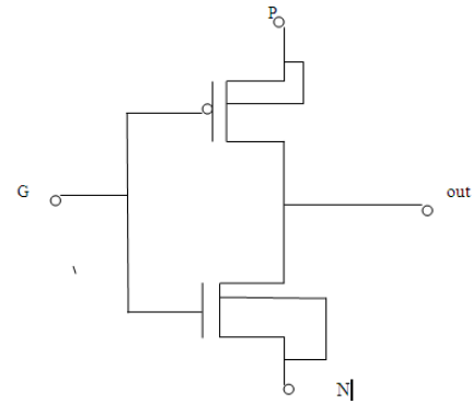
Fig.8 Basic GDI cell
