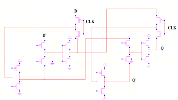
Fig.10 D flip-flop using GDI
