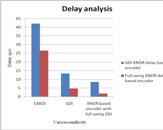
Fig.14 Delay analysis
