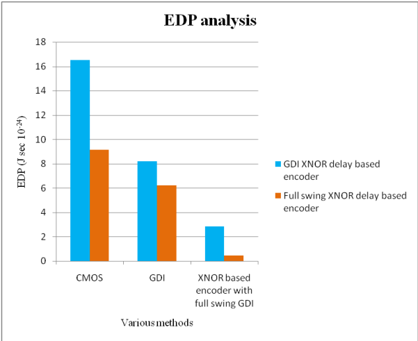
Fig.17 EDP analysis
