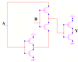
Fig.9 XNOR using gate diffusion input (GDI)
