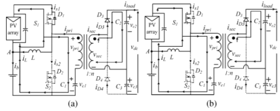
Fig. 5. Equivalent diagram of TCDIC when I_L is negative (a) Mode I (b) Mode II.
