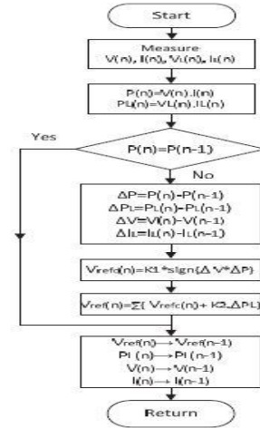
Fig. 8. RCC flow-chart
