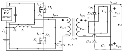
Fig. 3. Equivalent diagram of TCDIC in mode I and I_L is positive.
