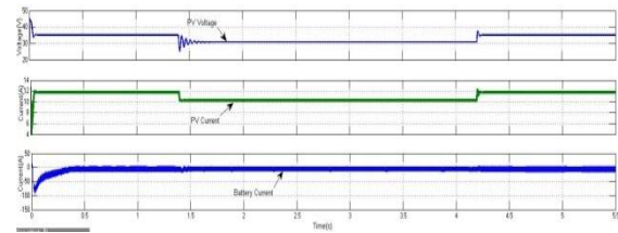
Fig. 13. i) Voltage of PV and Currents of PV and battery
