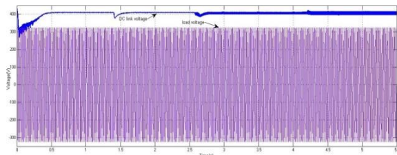
Fig. 12. ii) Voltages of DC link and load
