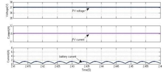
Fig. 11. i) Voltage of PV and Currents of PV and battery
