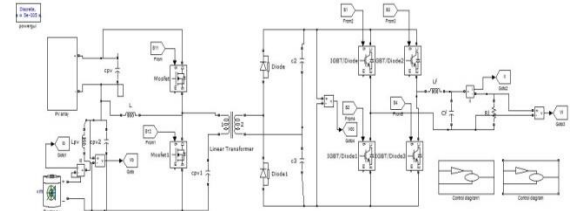
Fig. 9. Simulation Diagram.
