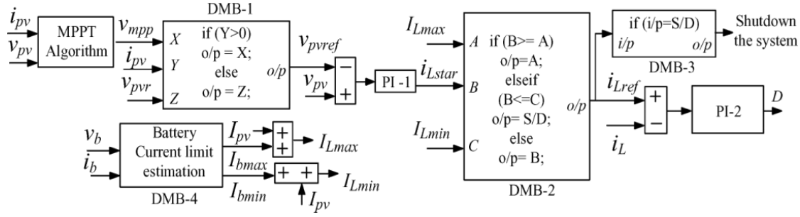
Fig. 6. TCDIC control structure
