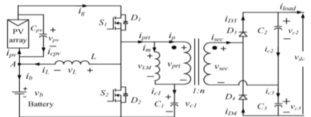
Fig. 1. TCDIC Circuit
