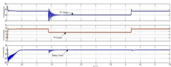
Fig. 12. i) Voltage of PV and Currents of PV and battery
