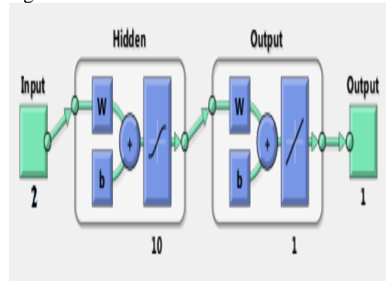
Fig. 6. structure of ANN for MPPT
