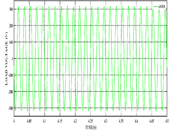
Fig. 14(c). Inverter output voltage
