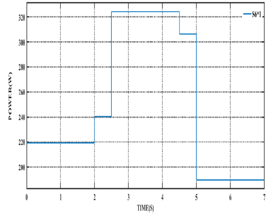
Fig. 3(a). Power performance of series configuration
