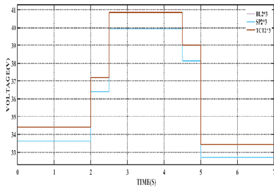
Fig. 2(c). voltage performance of 2*3 configuration
