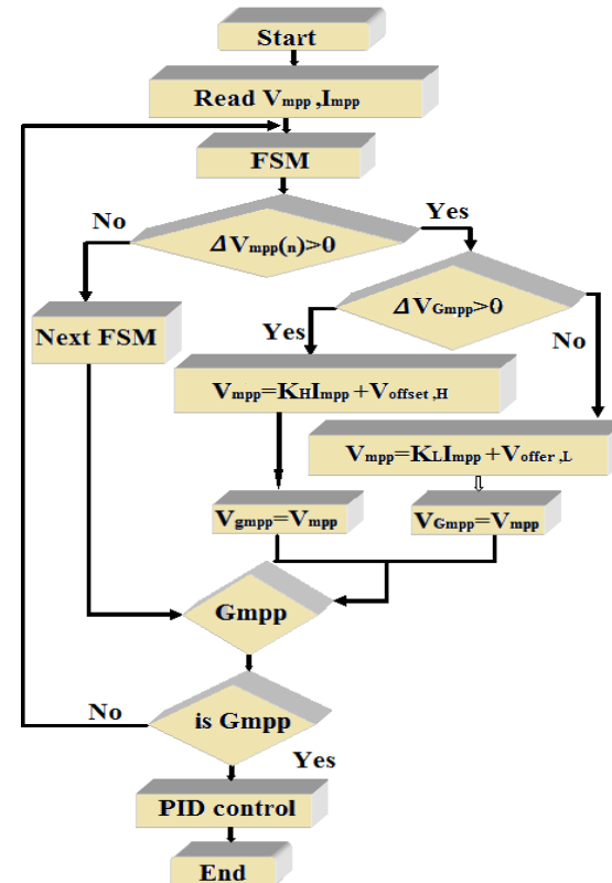
Fig. 9. Flow chart of FSM as MPPT From the flow chart it is noted that V_{\text{mpp}} and I_{\text{mpp}} are given as input to FSM and V_{\text{Gmpp}} is considered as T. From the Figure 9 it is noted that FSM finds the V_{\text{Gmpp}} for a given PV panel voltage and current. The V_{\text{Gmpp}} is
