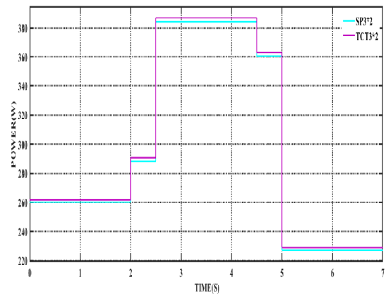
Fig. 3(b). Power performance of 3*2 configuration
