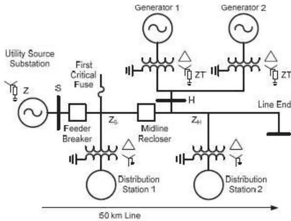
Fig. 3. Test System.
