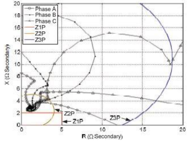
Fig. 6. Impedance plot
