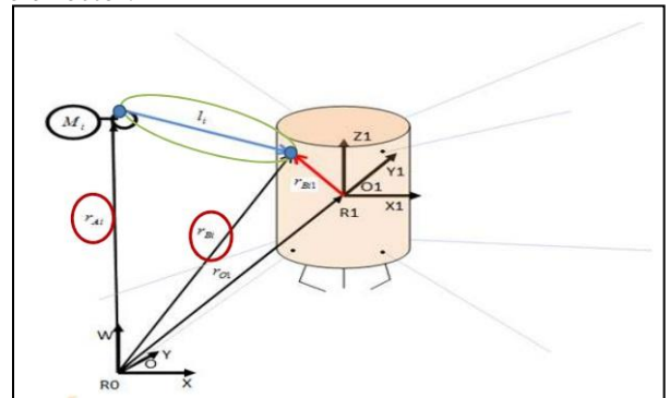
Fig. 3: General Diagram of the system As shown in Fig.3, the lengths l_i of the cables are:
