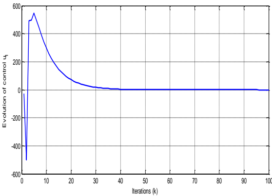
Fig. 7. Evolution of u_1(k) .
