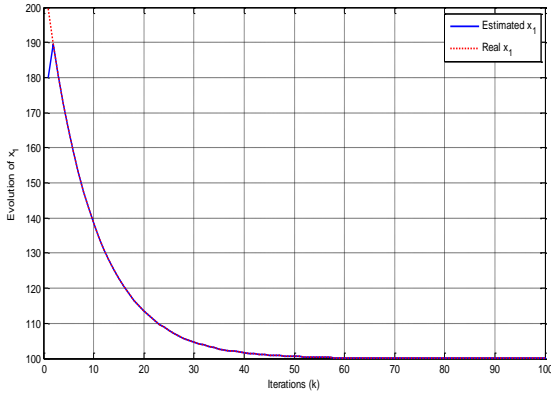
Fig. 6. Response of real x_1(k) and its estimate.
