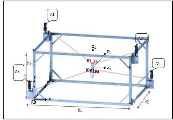
Fig 2. Cables Robot with 4 motors (under-actuated mode).
