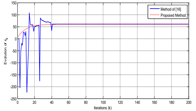
Fig. 9. Response of \hat{x}_4(k) .
