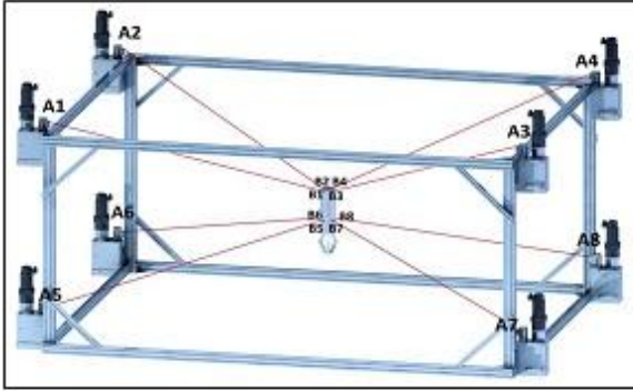
Fig.1. Cables Robot with 8 motors.
