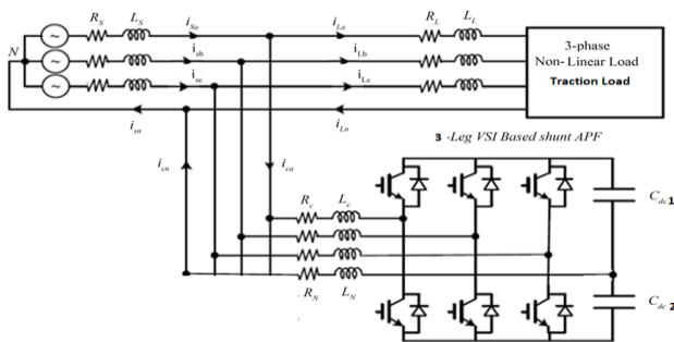
Fig.1. 3phase, four wire, Shunt APF with Traction Non-linear load
