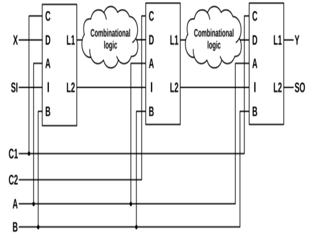
Fig. 2 Latch Based Scan Chain Organization
