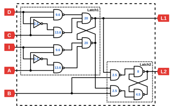
Fig. 3 Gate Level Schematic of Original LSSD
