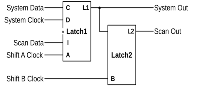
Fig. 1 Single Latch LSSD Using Shift Register Latch
