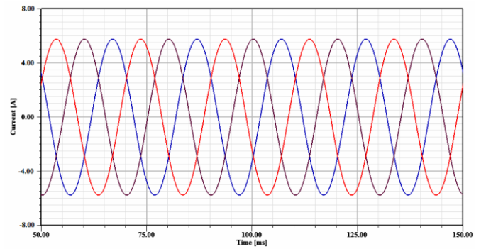
Fig. 11. Three-phase current waveform
