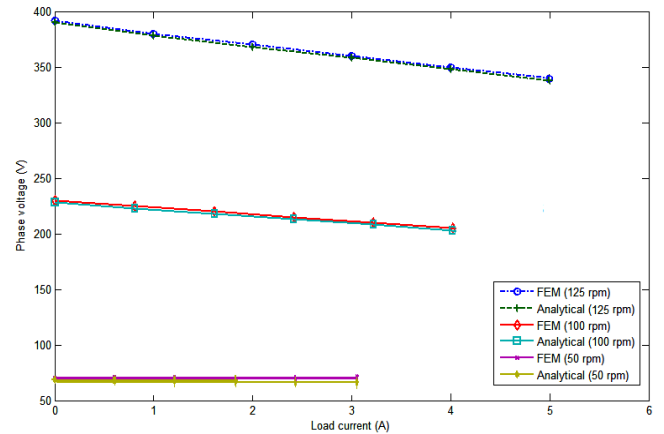
Fig. 12. Variation of phase voltage with respective to load current for various speeds of generator
