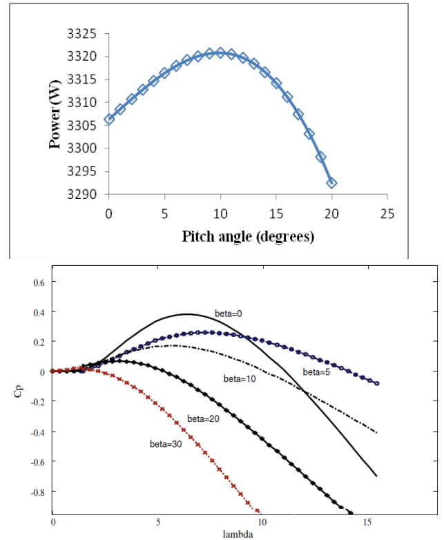
Fig. 3. C_p variations versus lambda and beta
