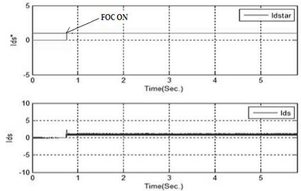
Fig. 8. Reference and Estimated dq-axis currents vs Time
