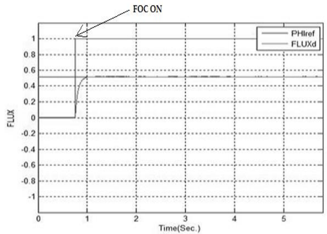
Fig. 7. Reference and Estimated Flux vs Time
