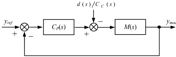
Fig. 2. Equivalent BMC main loop.
