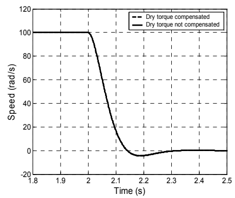
Fig. 11. Influence of the dry torque – BMC control.
