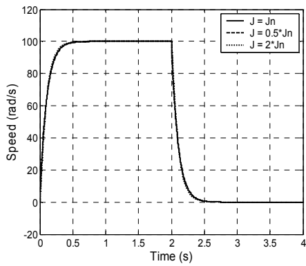
Fig. 8. BMC speed control – rotor inertia variation.
