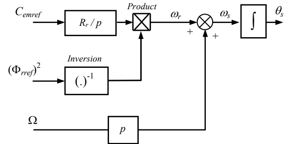
Fig. 5. Block of \theta_s estimation.
