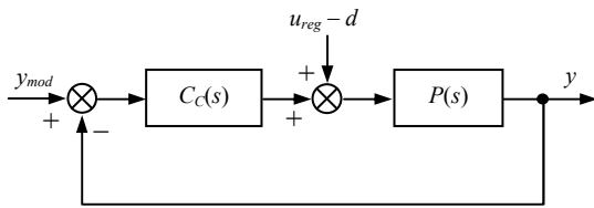
Fig. 3. Equivalent BMC secondary loop.
