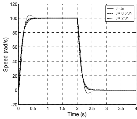
Fig. 7. Conventional speed control – rotor inertia variation.
