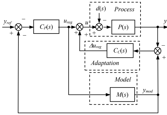
Fig. 1. Behaviour model control structure.
