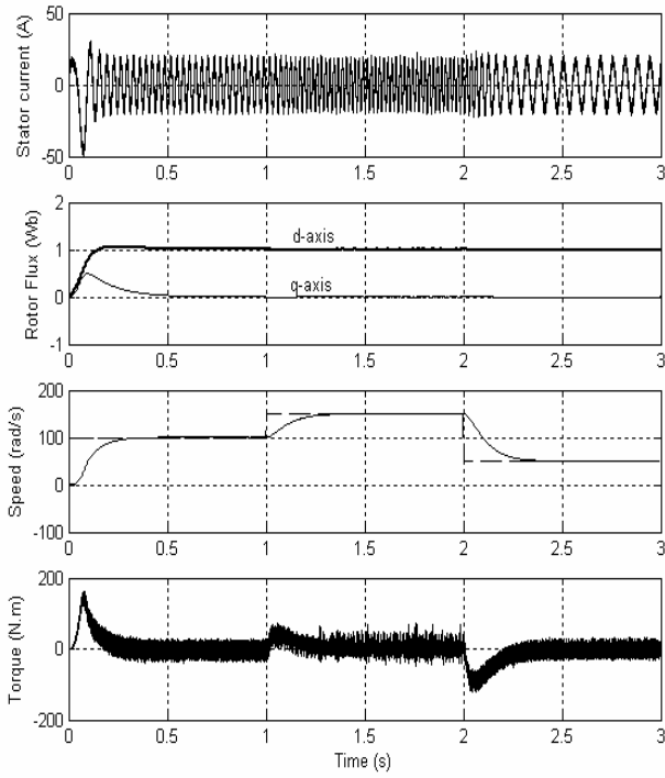
Fig. 6. BMC control of induction machine with speed reference variation (100, 150, 50 rad/s).
