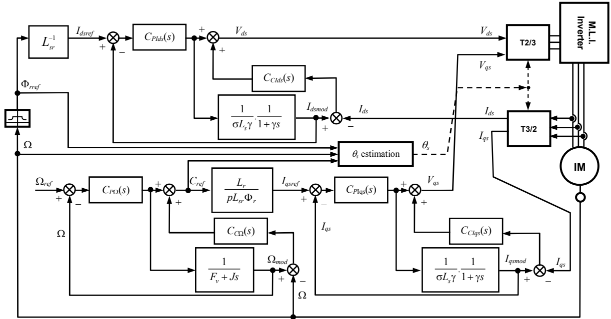
Fig. 4. Behaviour model control of an induction machine.
