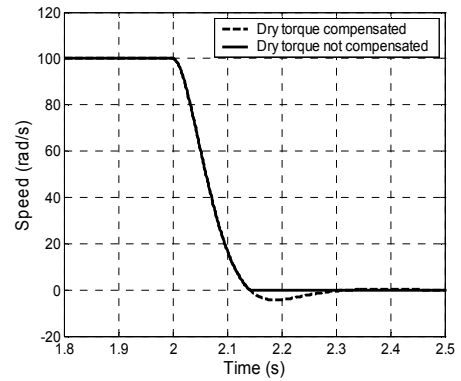
Fig. 10. Influence of the dry torque – conventional control.
