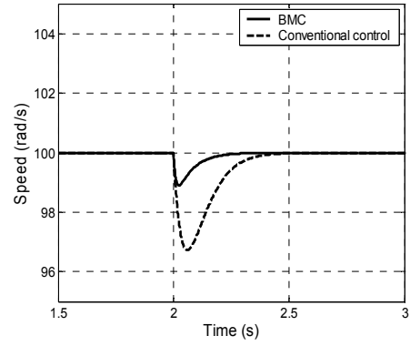
Fig. 9 Speed response –Application of a load torque (20 N.m) at t = 2s .
