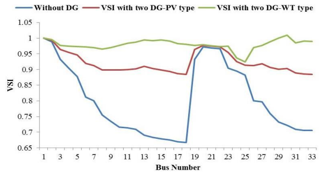
Fig.6. VSI of IEEE 33 bus system with two DG units
