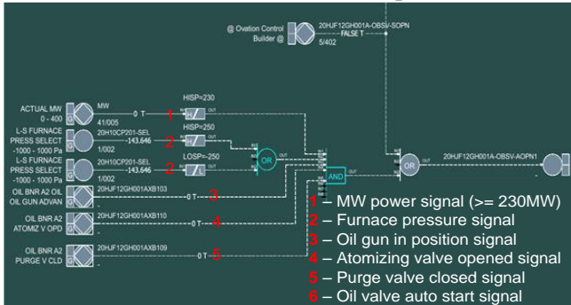
Fig. 5. Improvement of the oil valve logic for the oil valve in automatic opening
