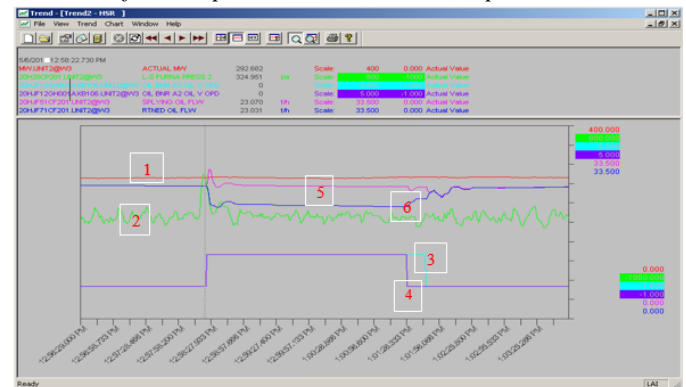
Fig. 8. Automatical opening of the oil valves when the furnace pressure more than +250pa
