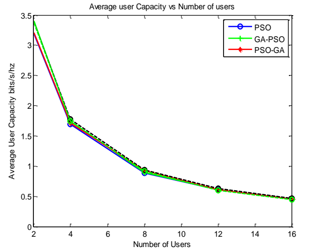
Figure 8. Average user capacity vs number of users
